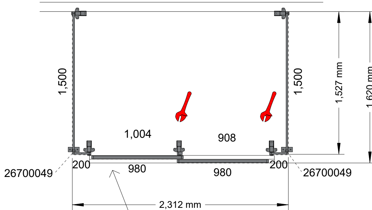
Hasp and staple lock (padlock to be supplied by others).
